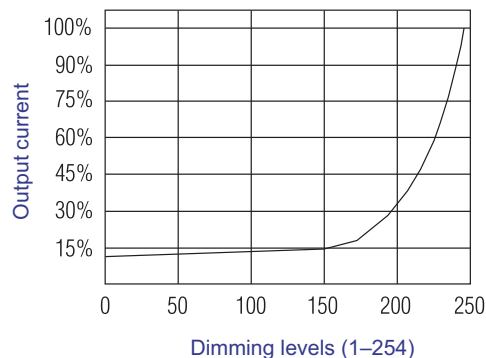
Dimming curve
