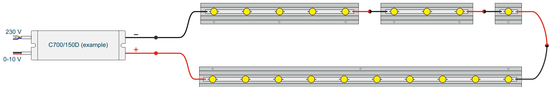
Example 1: More profiles powered by one converter
