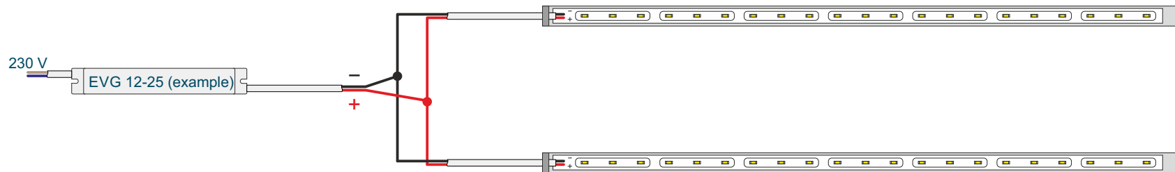
Example 2: two Mini Profiles operated with 12 volts
